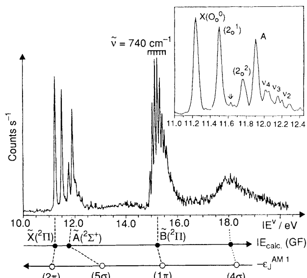
Fig. 2 He I PE spectrum of HC≡C–N≡C [calibrated with 2 P 3/2 (Ar) = 15.76 eV] and its assignment based on correlated Green function ionization energies, IE_{i,v}^{calc.} (GF), and on Koopman's correlation, IE_{i,v} = -\epsilon_j^{AM1} , with eigenvalues from a fully geometry-optimized AM 1 calculation. Insert: expanded record between 11.1 and 12.60 eV with assignment of the vibrational radical cation states observed according to anharmonic ab initio potential energy function calculations, 5c (cf. Table 1); the rather weak peak at 11.60 eV (↓) could be owing to traces of the acetylene cyanide isomer formed in the thermal fragmentation (see, text).
