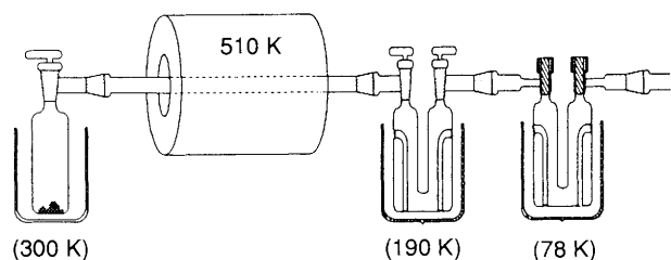
Fig. 1 Building block apparatus assembled for the 510 K thermolysis of the pentacarbonylchromium complex, for the fractionate condensation of side products in a 190 K intense cooling trap and for the isolation of acetylene isocyanide in a 78 K trap with Teflon valves. The photoelectron spectrometer (PES) connected is used both for the evaporation of the system and for the optimization of the reaction conditions and the product analysis.
